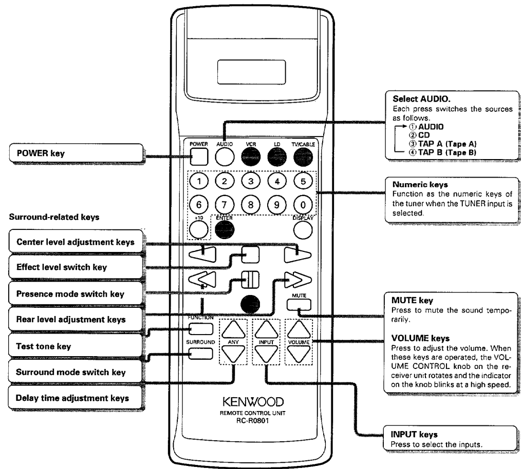
Model: RC-R0801 Infrared ray system
